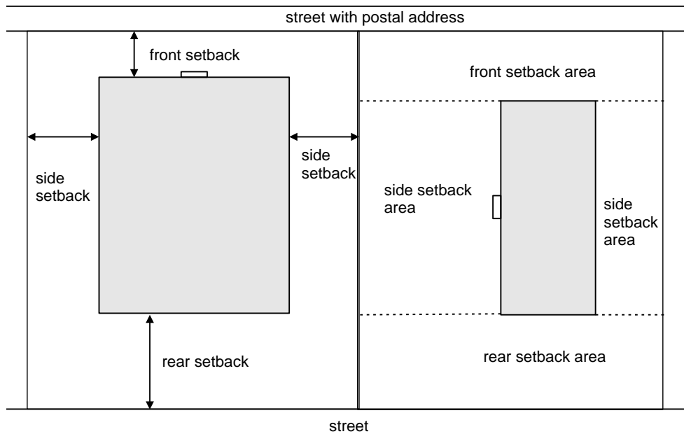
Figure 4 Through lot setback distances and areas.
