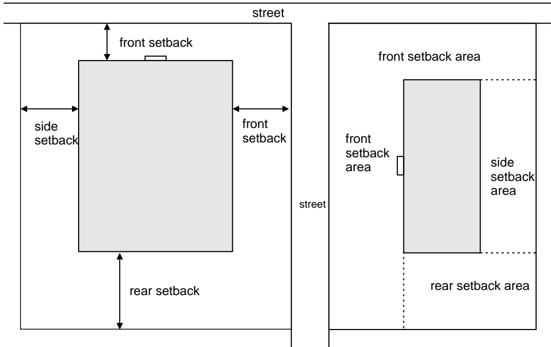
Figure 3 Corner lot setback distances and areas.
