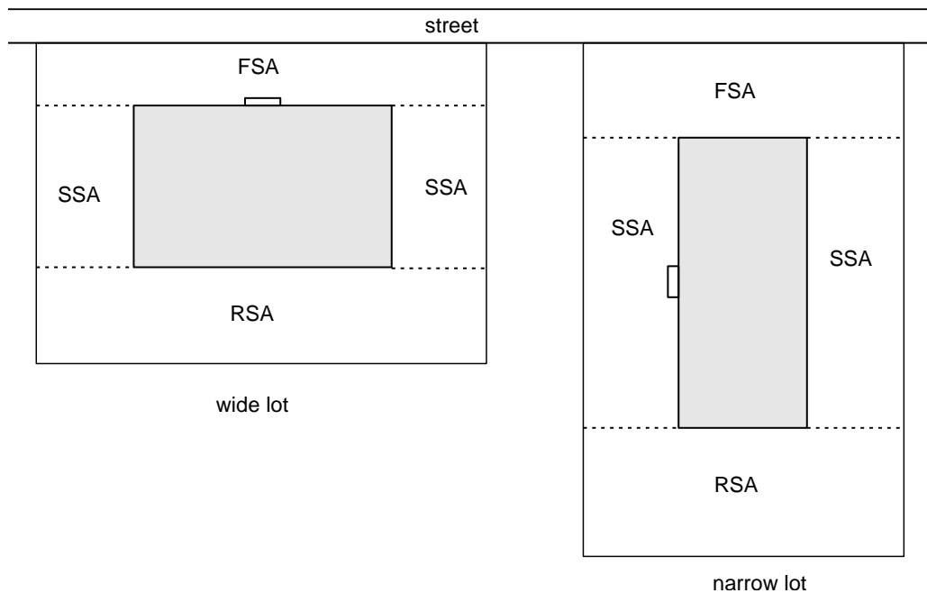
Figure 2 Wide and narrow lot setback areas. FSA: Front Setback Area, SSA: Side Setback Area, RSA: Rear Setback Area
