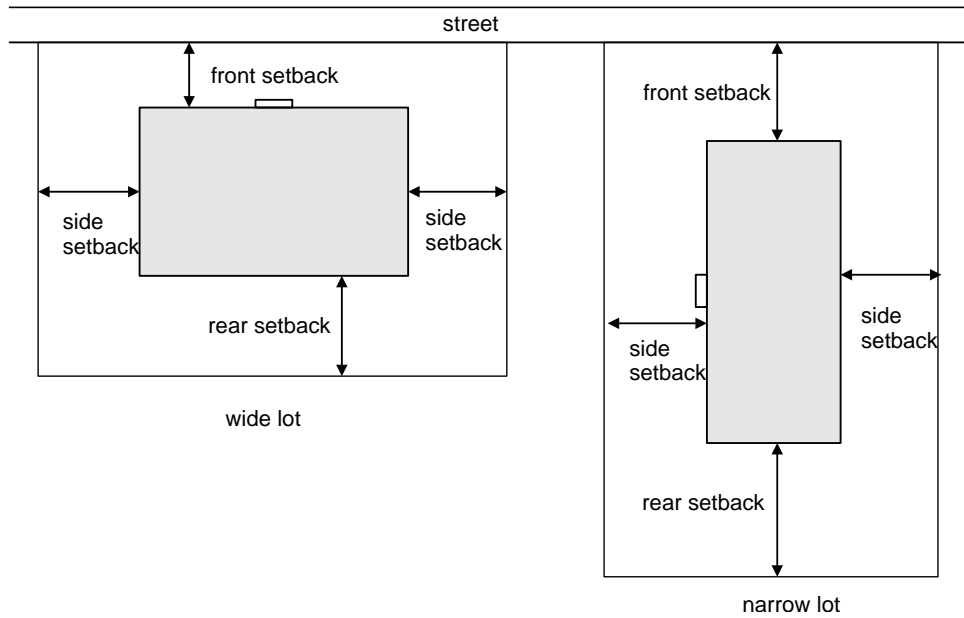
Figure 1 Wide and narrow lot setback distances.
