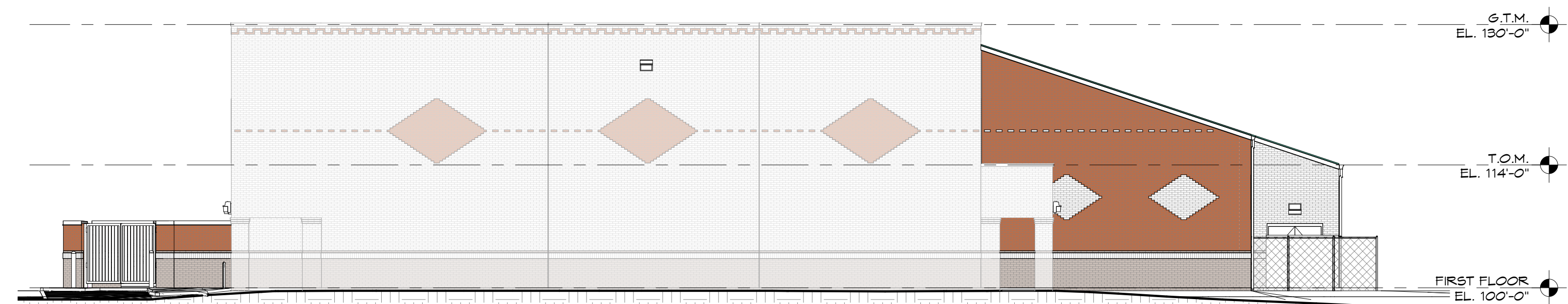
3 EAST ELEVATION 3/32" = 1'-0"
