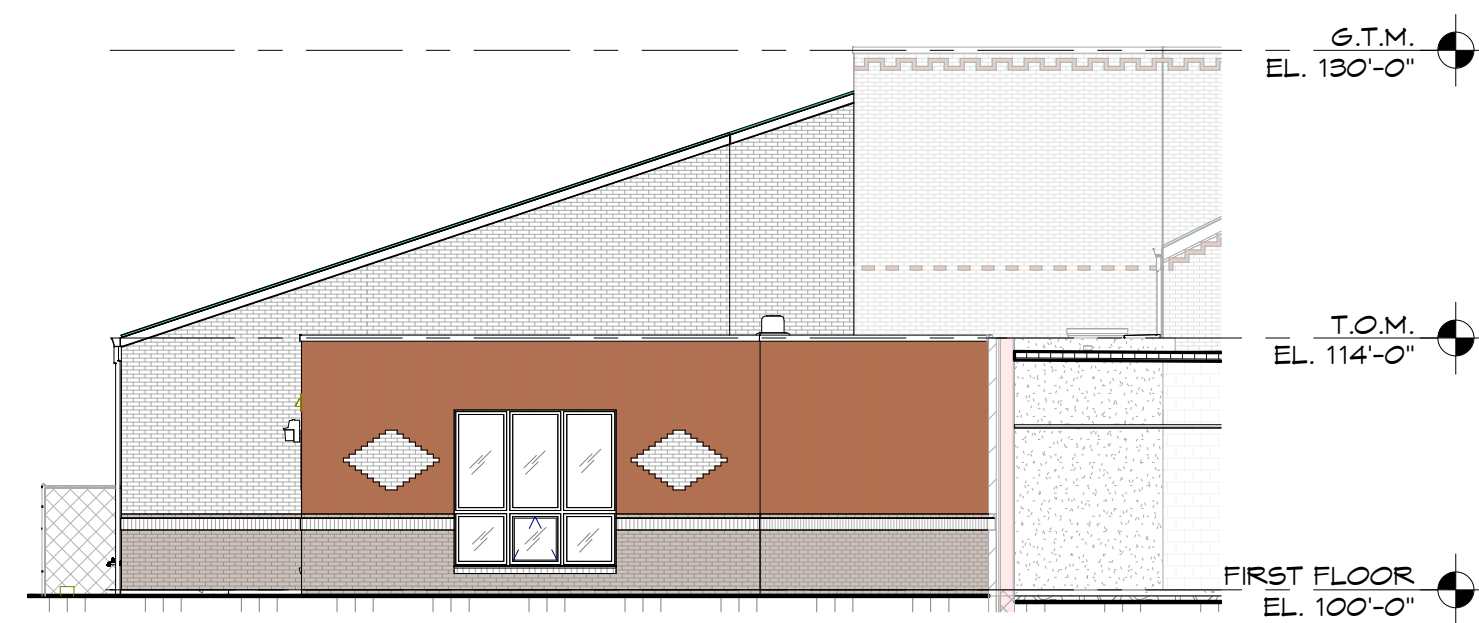
2 WEST ELEVATION 3/32" = 1'-0"
